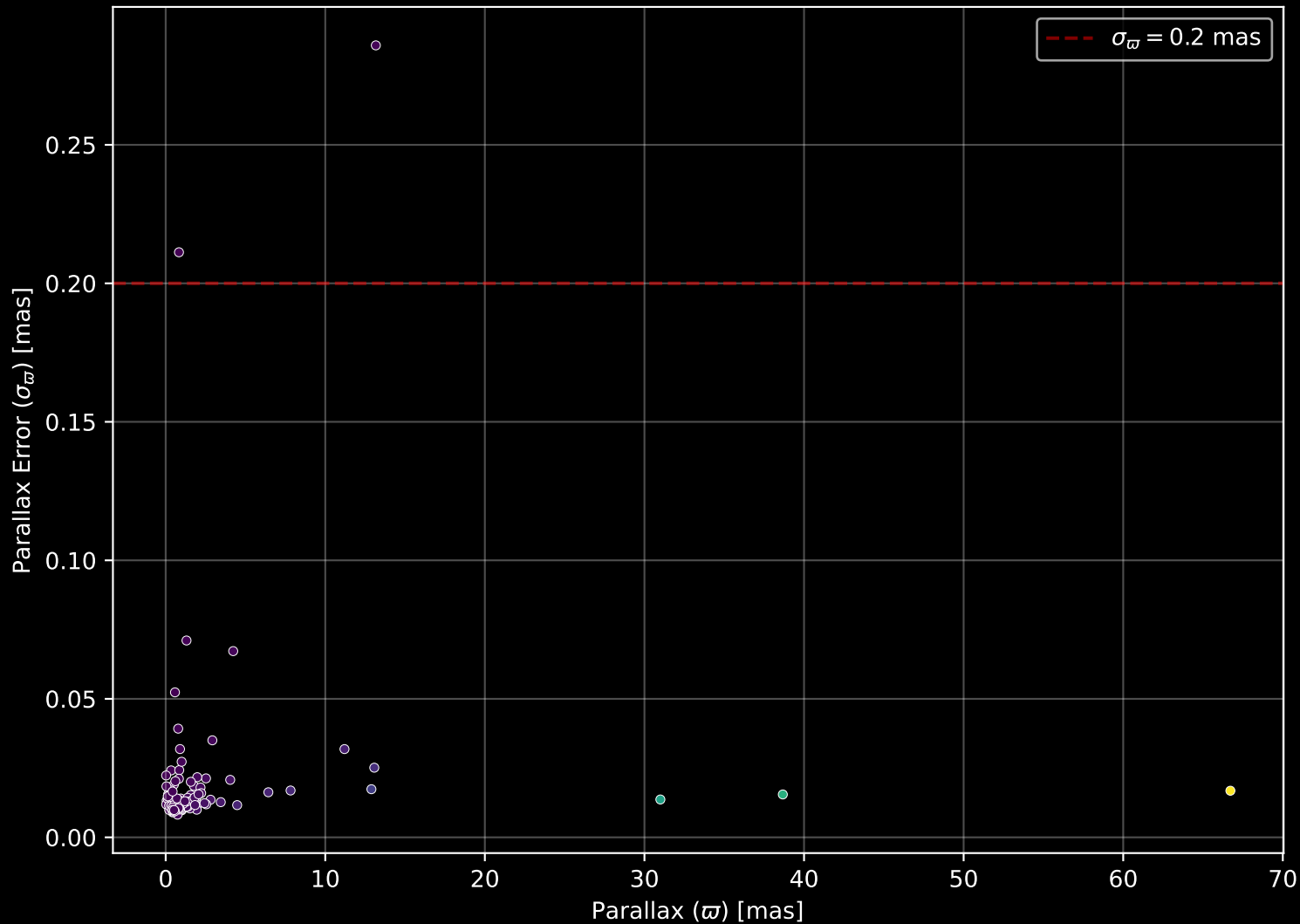
APOGEE DR17 Field: [135+30] Parallax Quality (n= 159)
