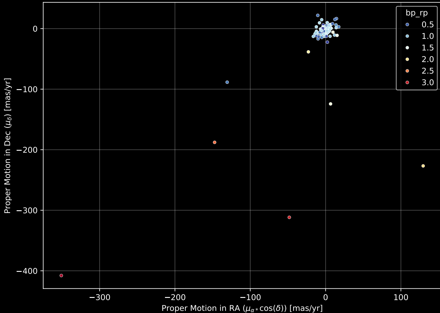
APOGEE DR17 Field: [135+30] Proper Motion Diagram (n= 159)
