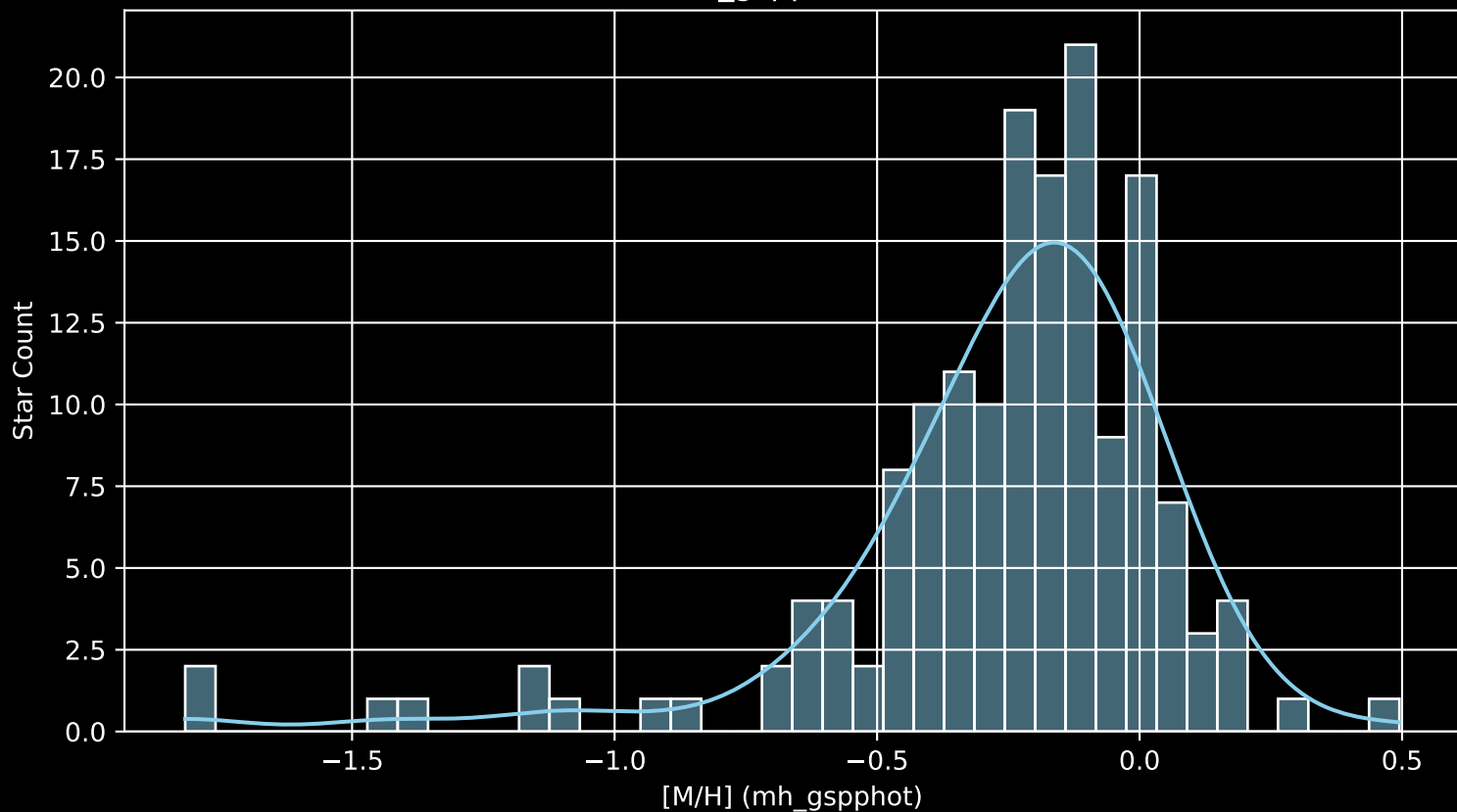
APOGEE DR17 Field: [135+30 [M/H] (mh_gspphot) (n= 159)
