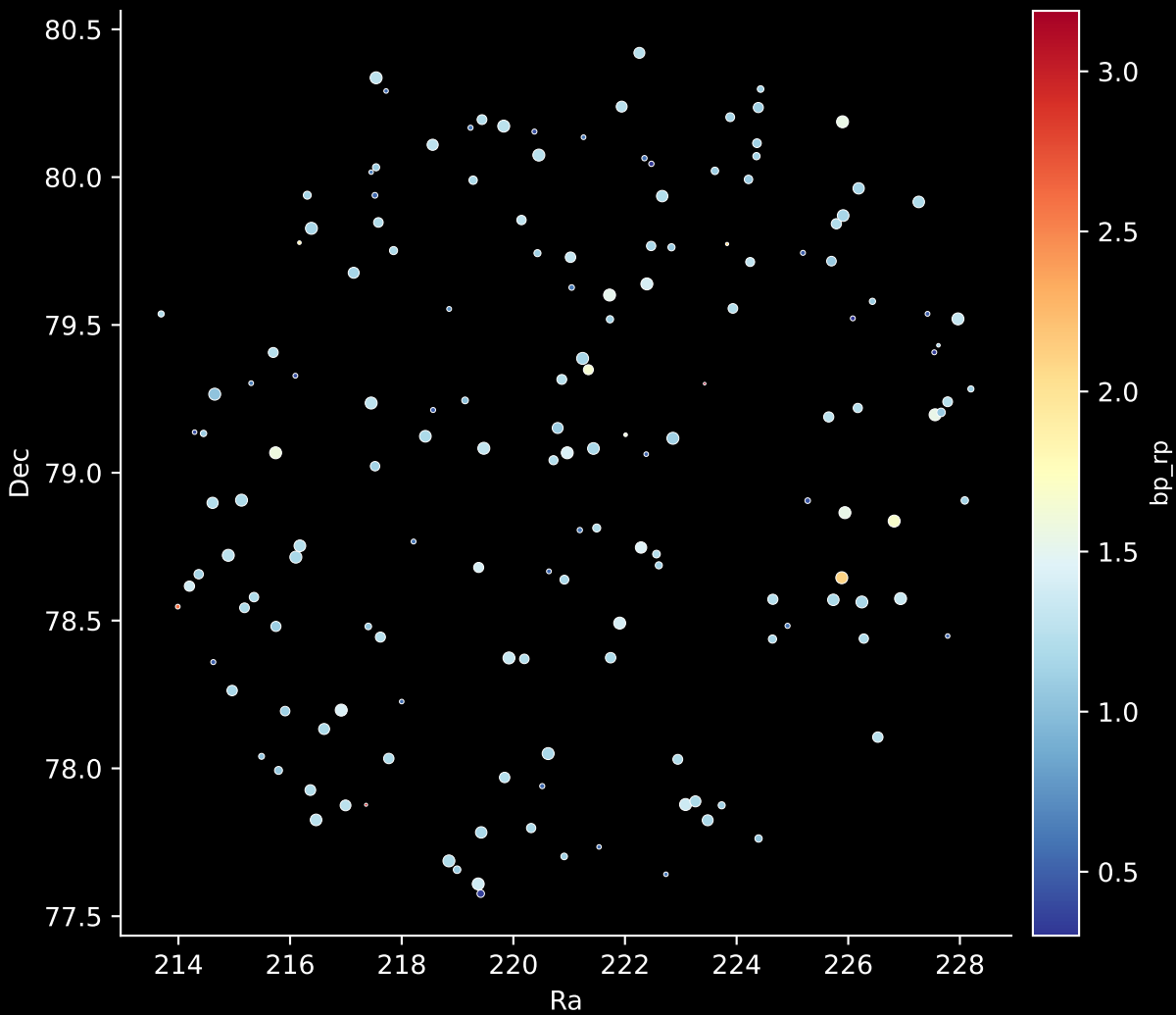
APOGEE DR17 Field: [135+30] Stars: 159
