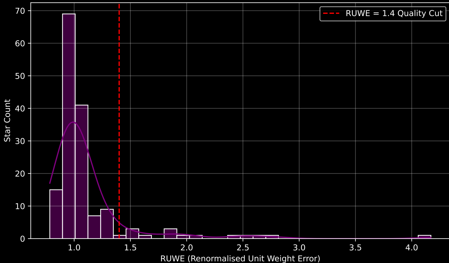
GAPOGEE DR17 Field [135+30] RUWE Distribution (n= 156)
